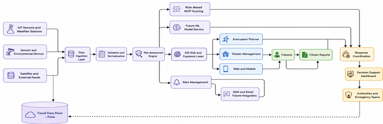
System architecture
